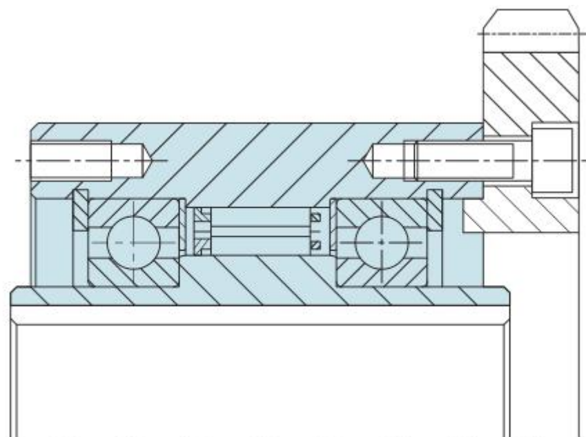
MOUNTING EXAMPLE
